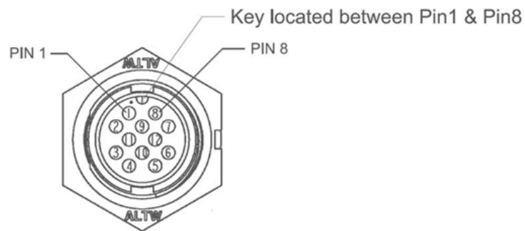
Figure 3-1: V200s pin-out assignments
