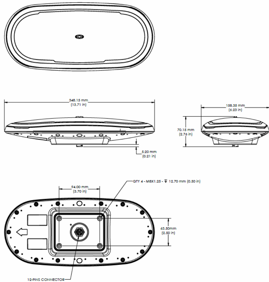
Figure 2-6: V200s dimensions
