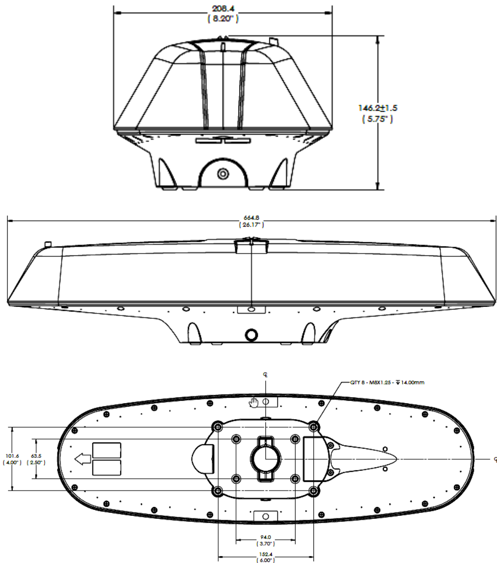
Figure 2-7: V123_V133 dimensions
