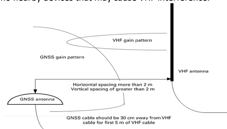
Figure 2-2: V123_V133 distance from nearby VHF radios
