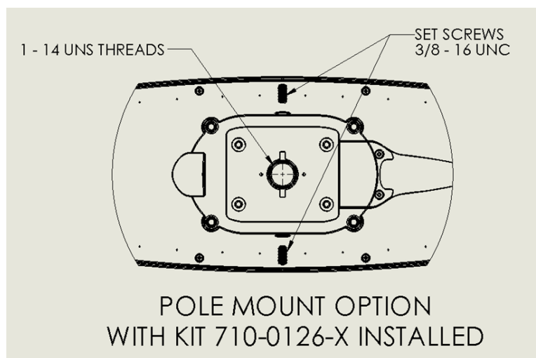
Figure 2-11: Pole-mounting specifications
