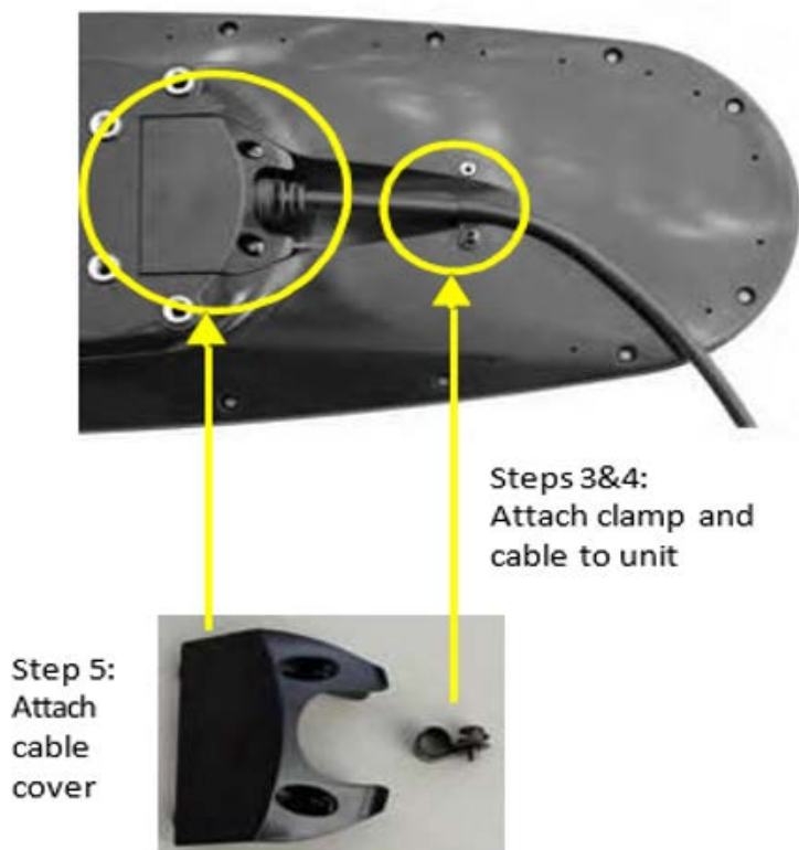
Figure 2-8: Connecting the serial power/data cable
